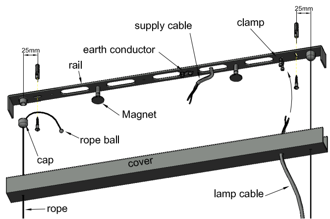
Canopy assembly
